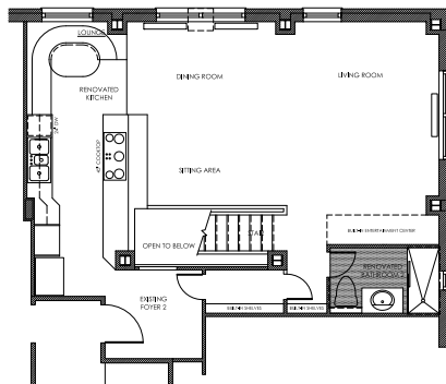
Upper Level Floor Plan
