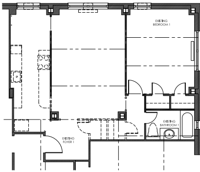
Lower Level Demolition Plan
