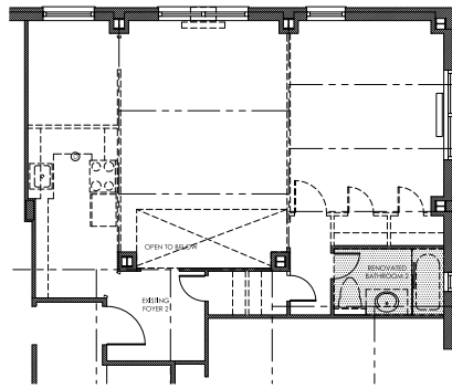
Upper Level Demolition Plan
